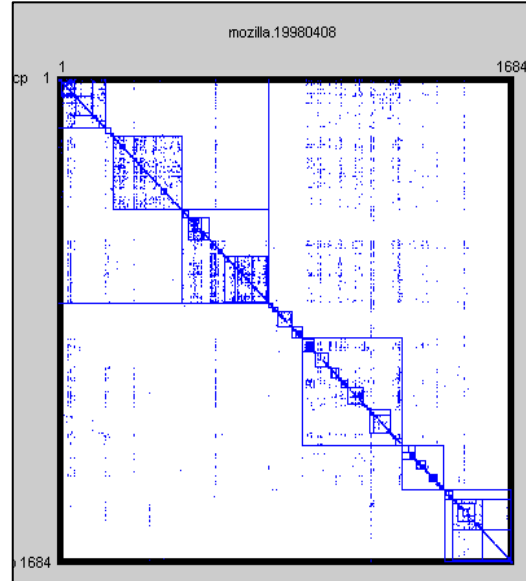
Figure 15: Mozilla DSM
