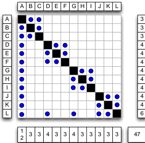
Figure 25: DSM of Hierarchy of Modules
